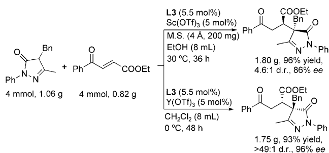
Scheme 1. The gram-scale synthesis of 3a that demonstrates the switch in enantioselectivity. M.S. = molecular sieves.
